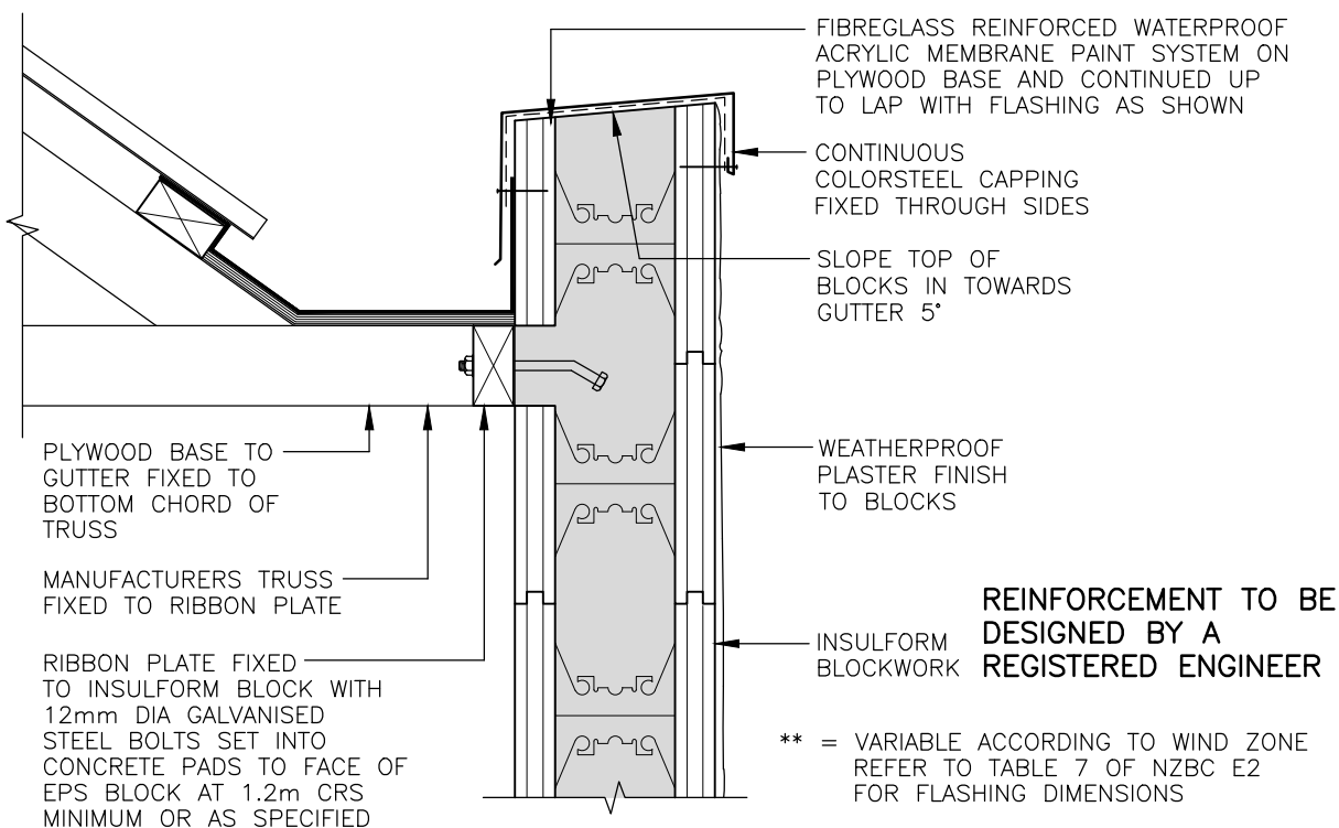
INTERNAL GUTTER DETAIL (ACRYLIC PAINT MEMBRANE GUTTER)
